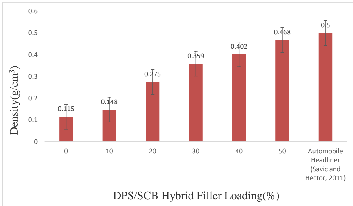
Figure 8: Density of DPS/SCB composites
