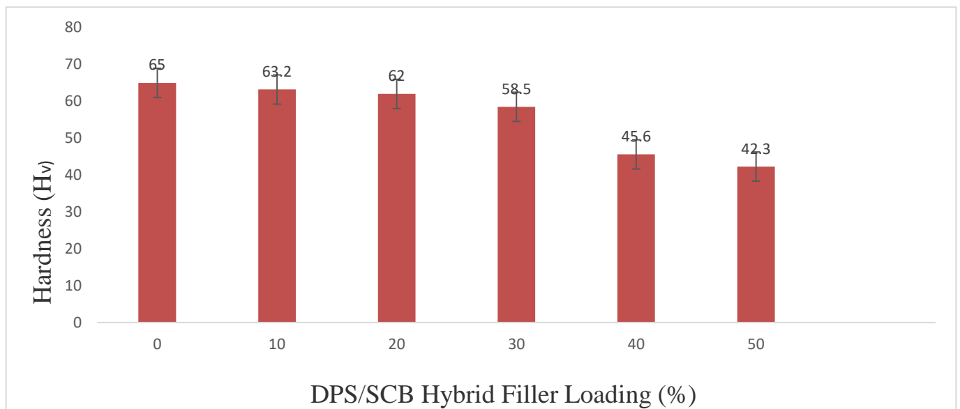
Figure 6: Effect of material loading on Hardness of DPS/SCB/ PP hybrid Composite
