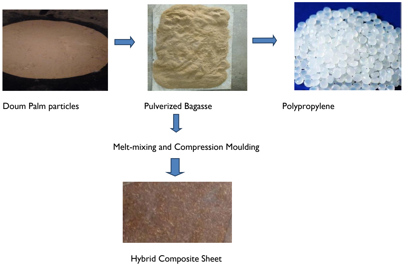
Figure 3: Flow chart for the Production of Hybrid Composite
