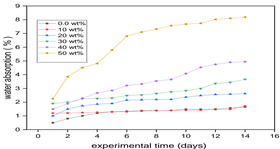
Figure 7: Percentage water absorption of DPS/SCB composites
