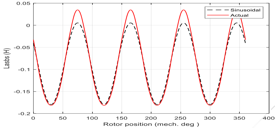
Figure 11: Mutual inductance between distributed stator winding, for phase A and phase B
