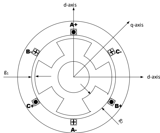
Figure 2: Three-phase four-pole Synchronous reluctance machine
