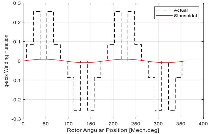
Figure 8: Fundamental components of q-axis cage winding expression, showing the actual and sinusoidal
