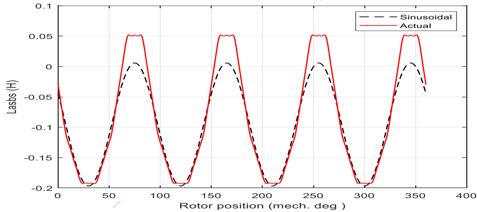
Figure 12: Mutual inductance between concentrated stator winding, for phase A and phase B
