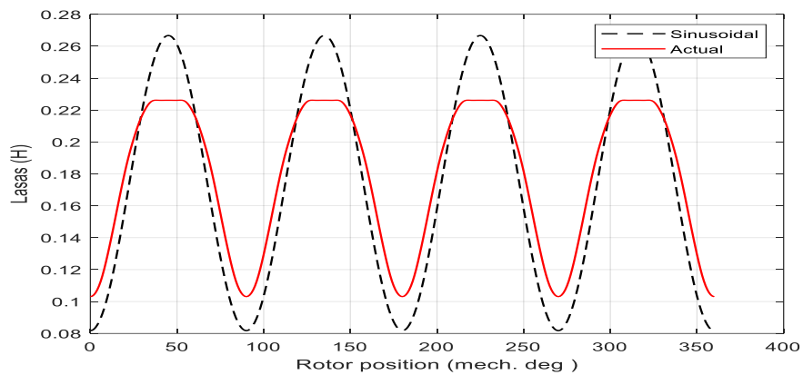
Figure 9: Self-inductance of distributed stator windings, for phase A
