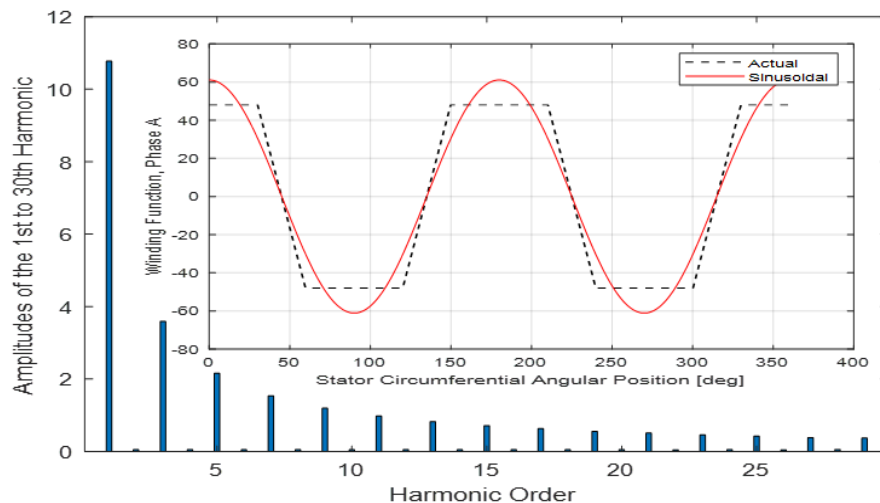
Figure 5: Phase A winding function of a 12-slot concentrated stator winding showing the actual, sinusoidal and the harmonic spectrum
