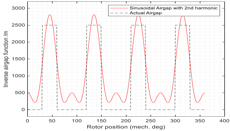
Figure 6: Inverse airgap function for actual and the sinusoidal considering only the second harmonic
