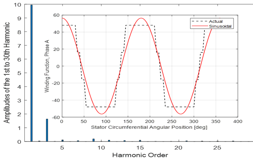
Figure 4: Phase A winding function of a 36-slot distributed stator winding showing the actual, sinusoidal and the harmonic spectrum
