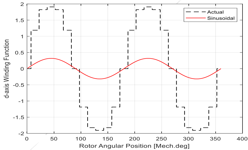
Figure 7: Fundamental components of d-axis cage winding expression, showing the actual and the sinusoidal
