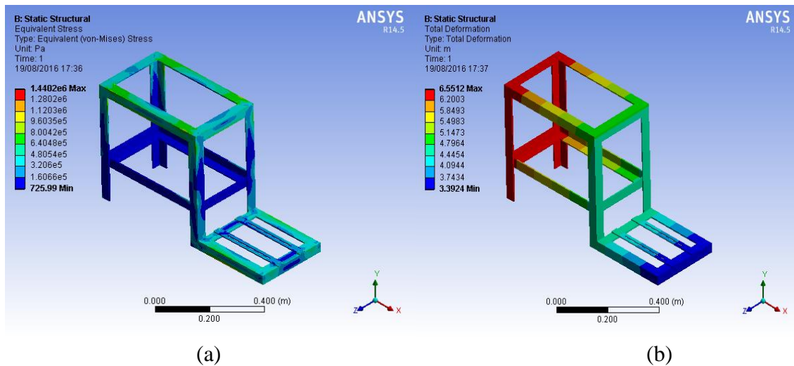
Figure 5: Stress (a) and deformation (b) analysis of machine tool frame
