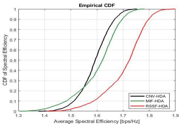
Figure 3: CDF Spectral Efficiency Over Average Spectral Efficiency
