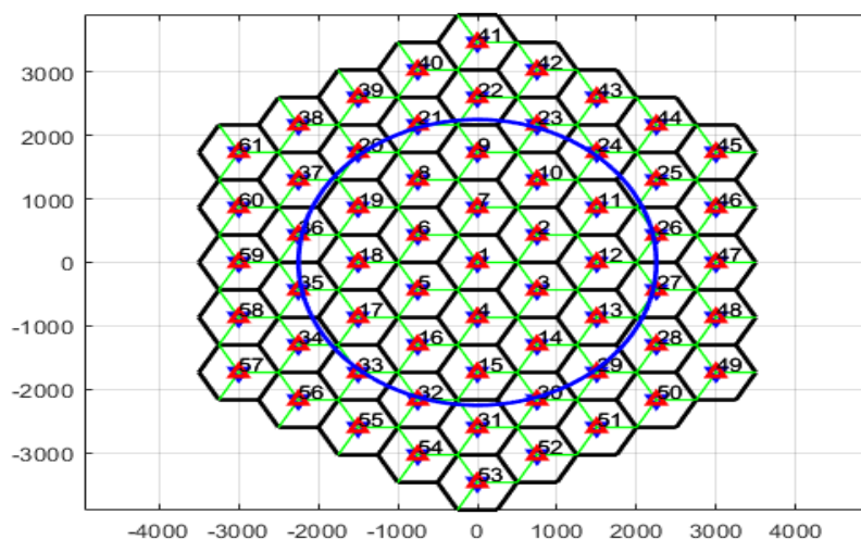
Figure 1: An illustration of the deployed scenario's clustered eNodeBs (Nkeleme et al., 2023)
