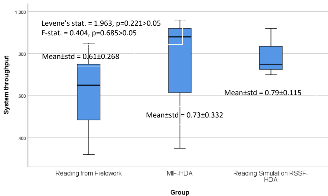
Figure. 7: Comparative result of readings from fieldwork, MIF-HAD, and Reading from Simulated RSSF-HDA of System throughput taken 0.2Mbps, 0.25Mbps, and 0.3Mbps respectively. The result (figure. 7) shows that readings from fieldwork lie between 0.61 \pm 0.268 ; readings from MIF-HDA lie between 0.73 \pm 0.332 , while readings from simulated RSSF-HDA lie between 0.79 \pm 0.115 . The Fisher's estimate with an F-statistic value of 0.404 and associated probability value of 0.685 > 0.05 indicates that the variations were not significantly high. However, it was inferred that there is no significant difference in readings of system throughput from the fieldwork, MIF-HDA, and simulated RSSF-HDA. The ANOVA test result was confirmed meaningful and accurate by Levene's test (Levene's stat. = 1.963, p=0.221 > 0.05 ); thereby, confirming the homogeneity of the variances in the data series which is one of the key assumptions of a data series for ANOVA test.
